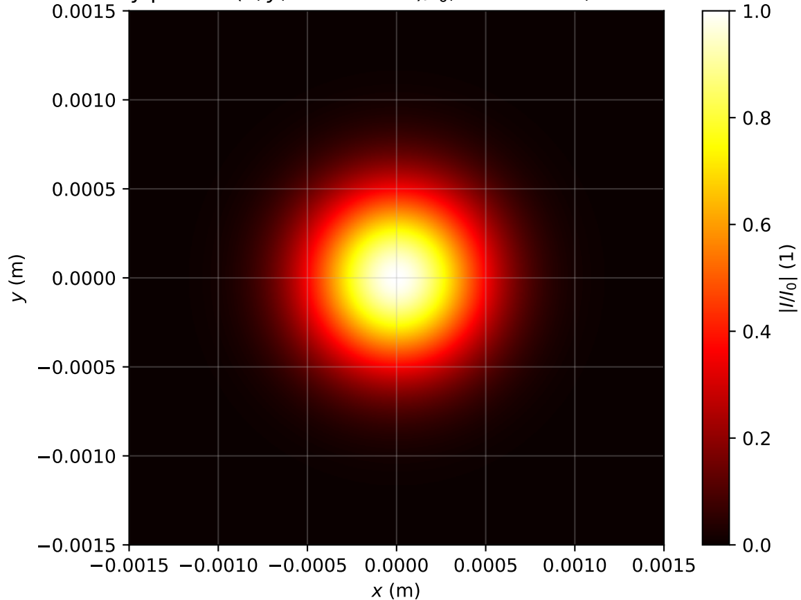
Intensity profile I(x, y, z = 0.000\text{m})/I_0 , Pin=0.8Pcr, artificial time
